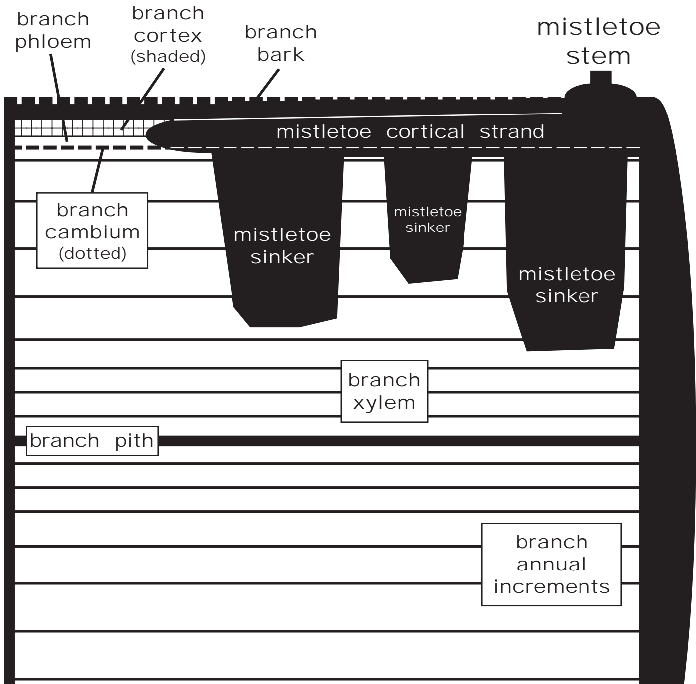
Figure 7: Simplified diagram along the longitudinal central axis of a branch with a mistletoe infection. Shown is a cortical strand and associated sinkers (mistletoe ray elements). The sinkers are maintained and grow outward with strand cambium aligned with the branch cambium.
