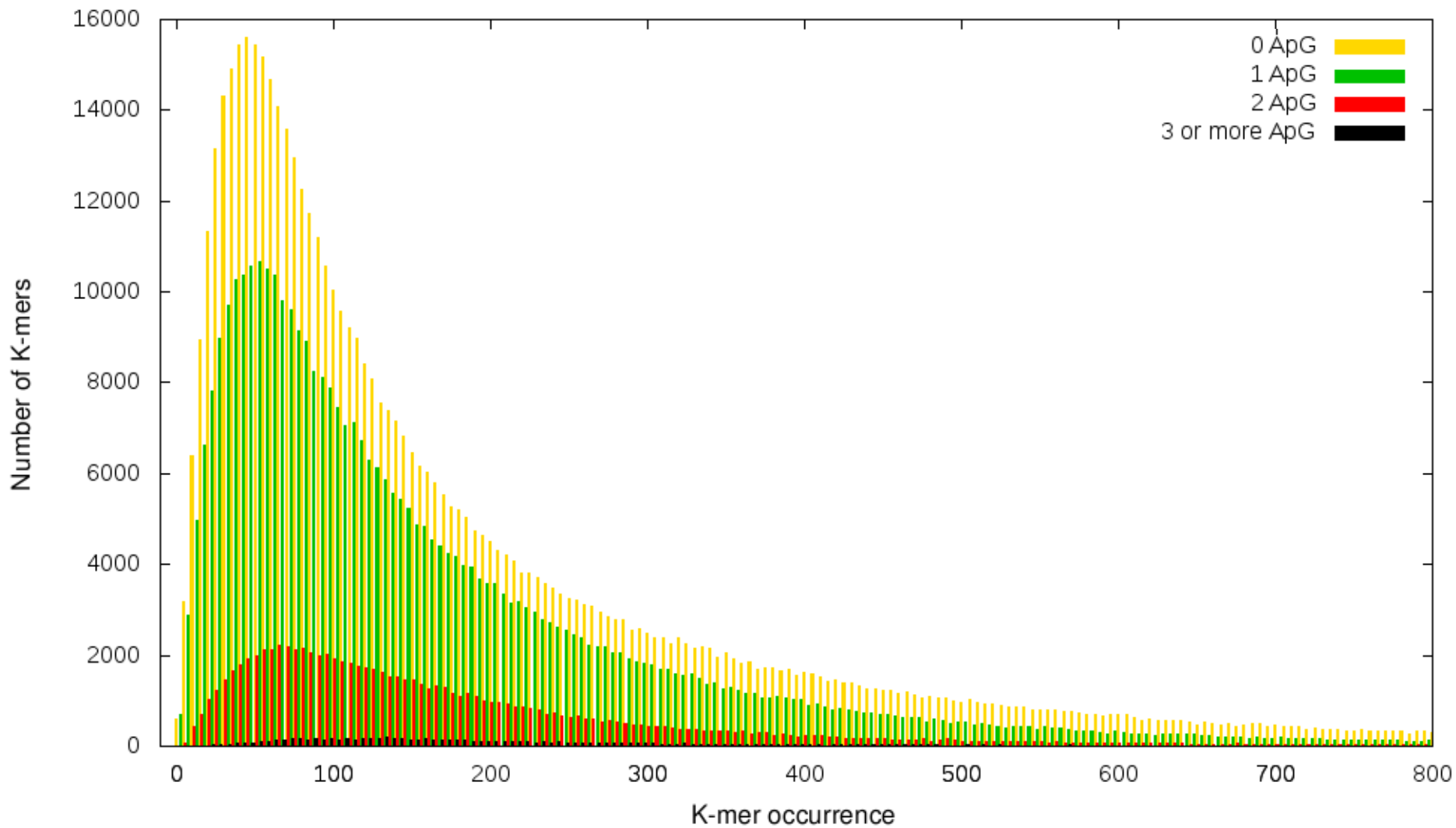
K-mers frequency distribution (K=10) - ApG partitioned
